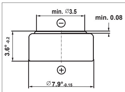
Diameter: 7.90 mm Height: 3.60 mm
