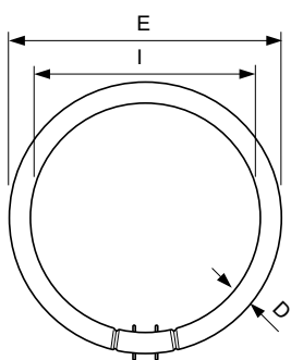
TL5-C 40W/840
