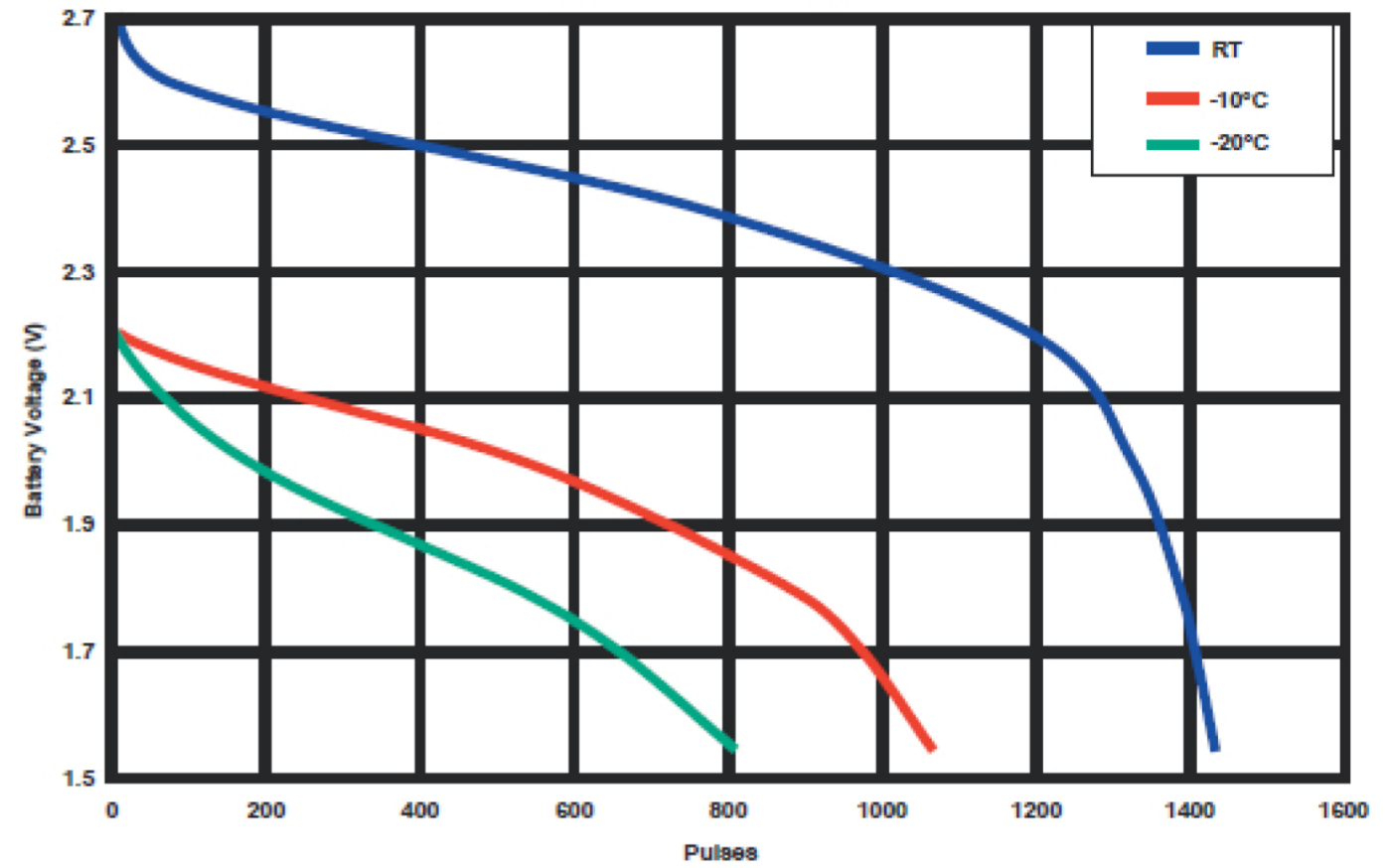
1.2 Amp, 3 sec on/ 7 sec off @ Various Temperatures
