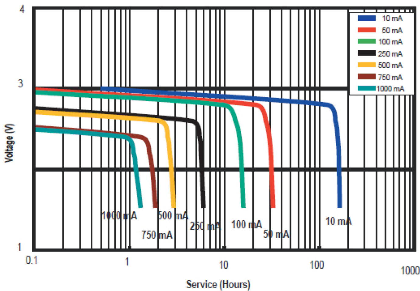
Continuous Discharge RT to 1.55 Volts
