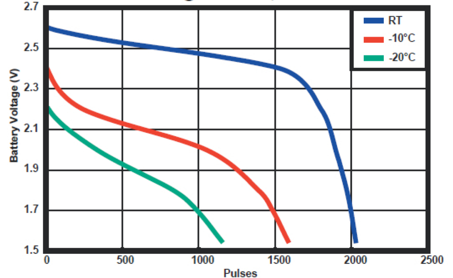
0.9 Amp, 3 sec on/27 sec off @ Various Temperatures
