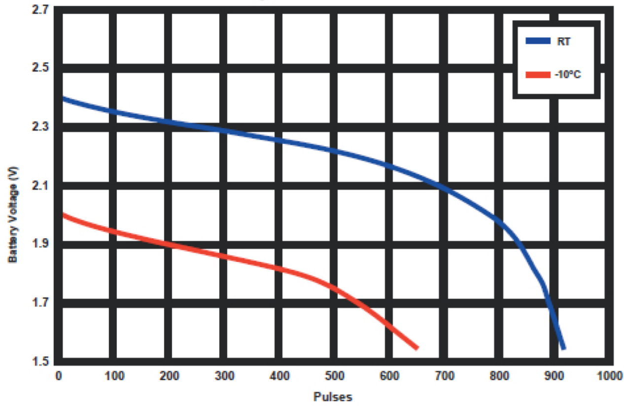
1.8 Amp 3 sec on/ 7 sec off @ Various Temperatures
