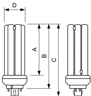
PL-T TOP 18W/830/4P A
