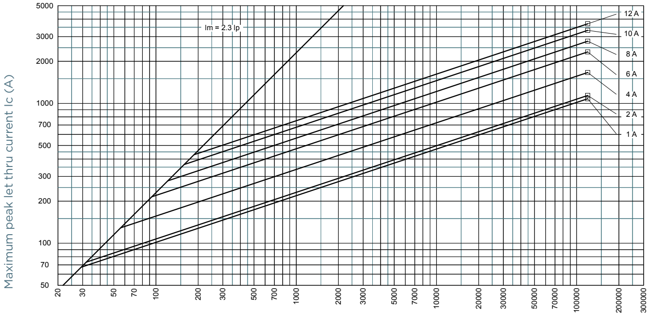
Size 10x38 400V aM with striker
