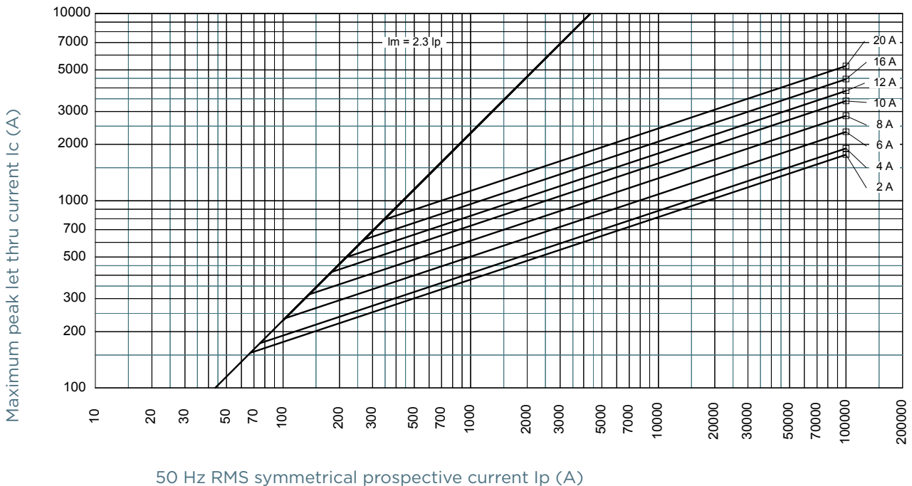
Size 10x38 400V aM with striker
