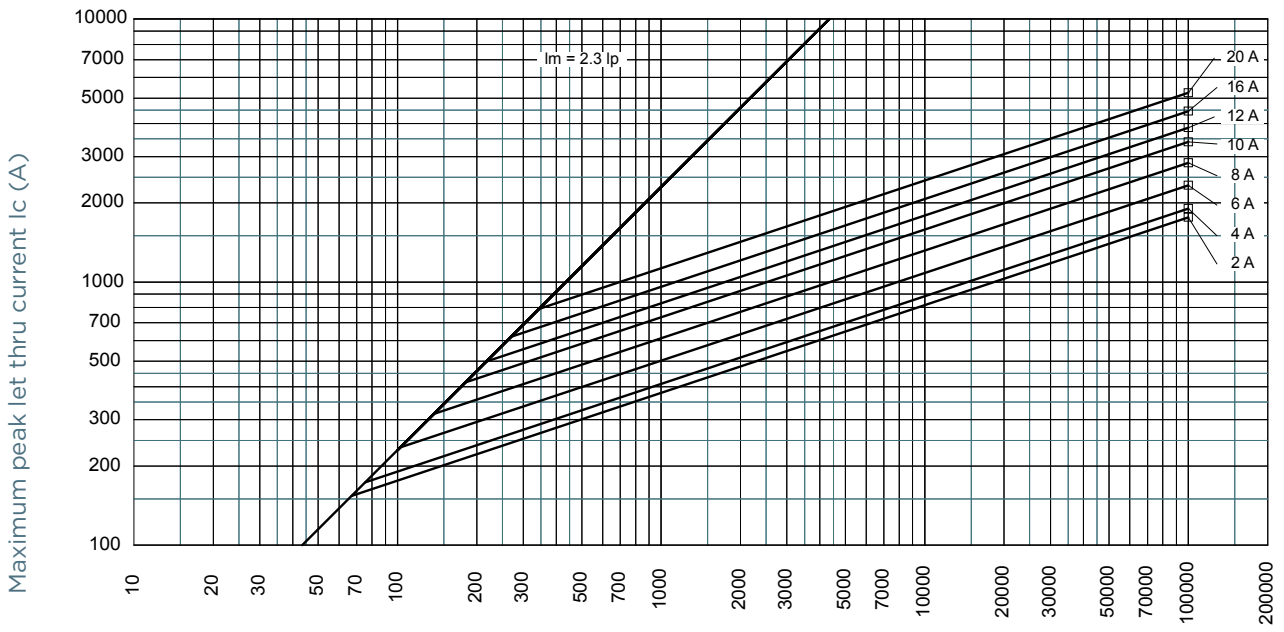
50 Hz RMS symmetrical prospective current I p (A)
