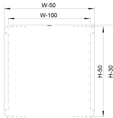
Mounting plate
