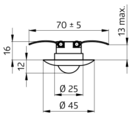
sensor head
