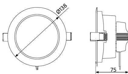
LEDDownlightRc-HZ R125
