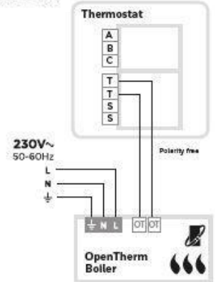
OpenTherm Boiler
