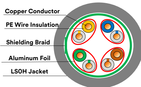
23AWG Cat.7 SFTP 4-Pair Solid Cable
