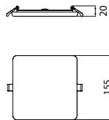
Pro-Space S 155x155mm 15W
