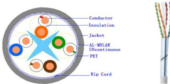
24AWG U/UTP 4-Pairs Cat.6 Solid Wire Cable
