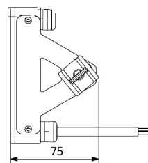
LEDflood-E Sensor
