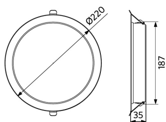
LEDDownlightCo-E Rd200
