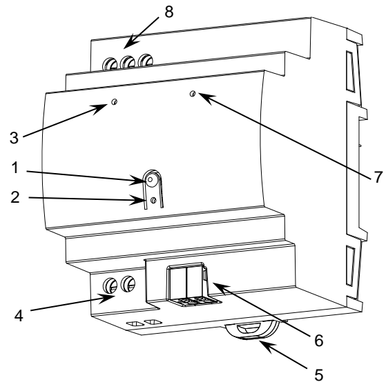
Figure 1: KUPSupply 320mA
