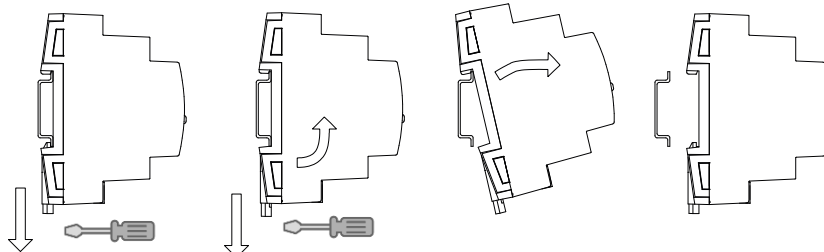
Removing KUPSupply 320mA from DIN rail:
