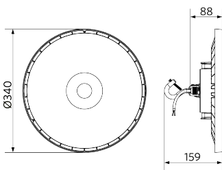
Dimensional_Drawing_HB_E3_110_140W.png
