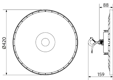
Dimensional_Drawing_HB_E3_180_220W.png
